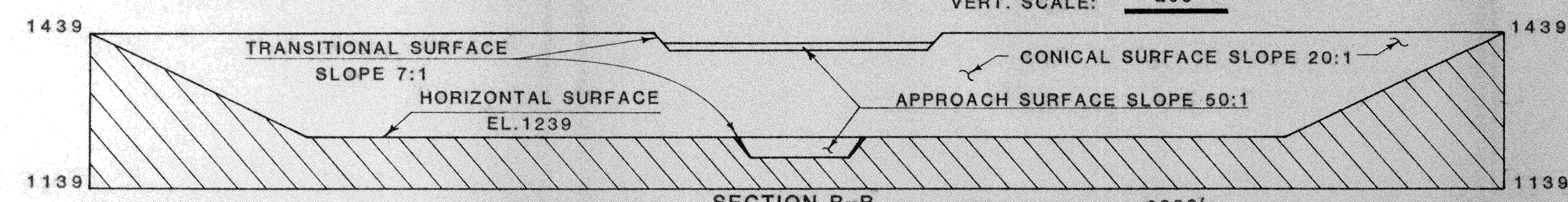
SECTION B-B
