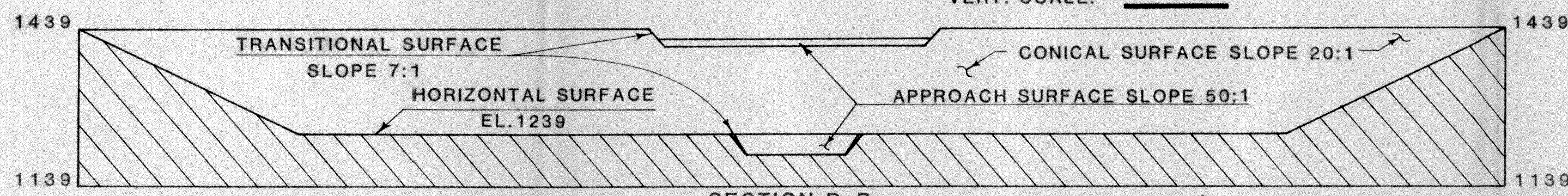
SECTION B-B
